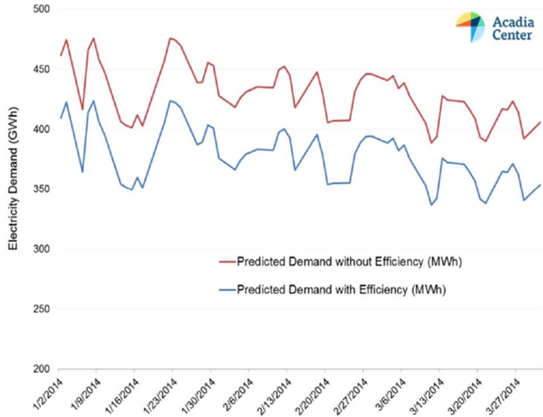
Figure 1: Daily Electricity Demand With and Without Efficiency
